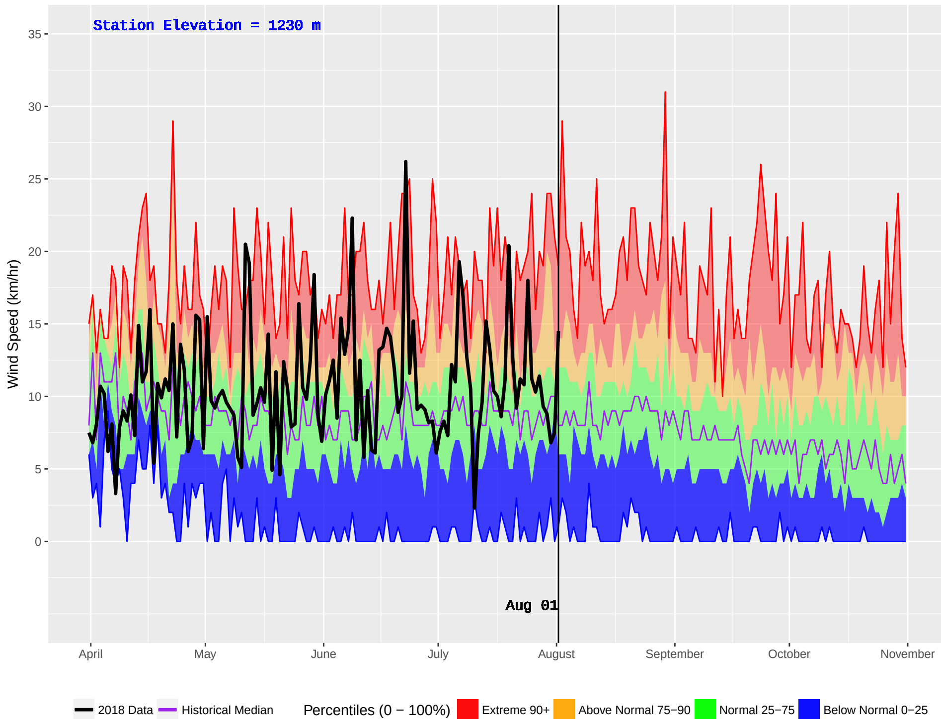
SLOCAN (406) : Historical (1992–2016) and Current (2018) Daily Wind Speed
