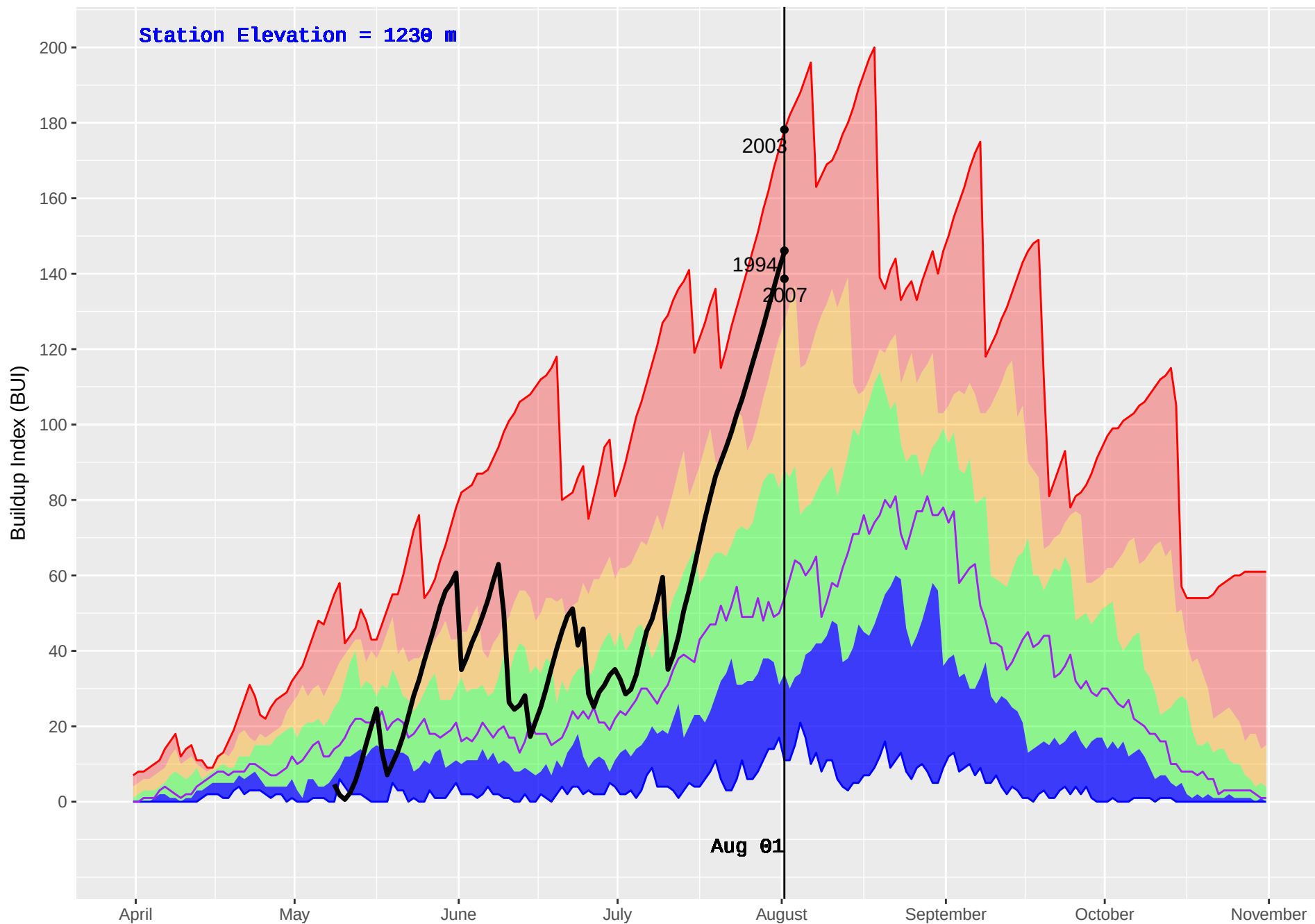
SLOCAN (406) : Historical (1992–2016) and Current (2018) Daily Buildup Index (BUI)
