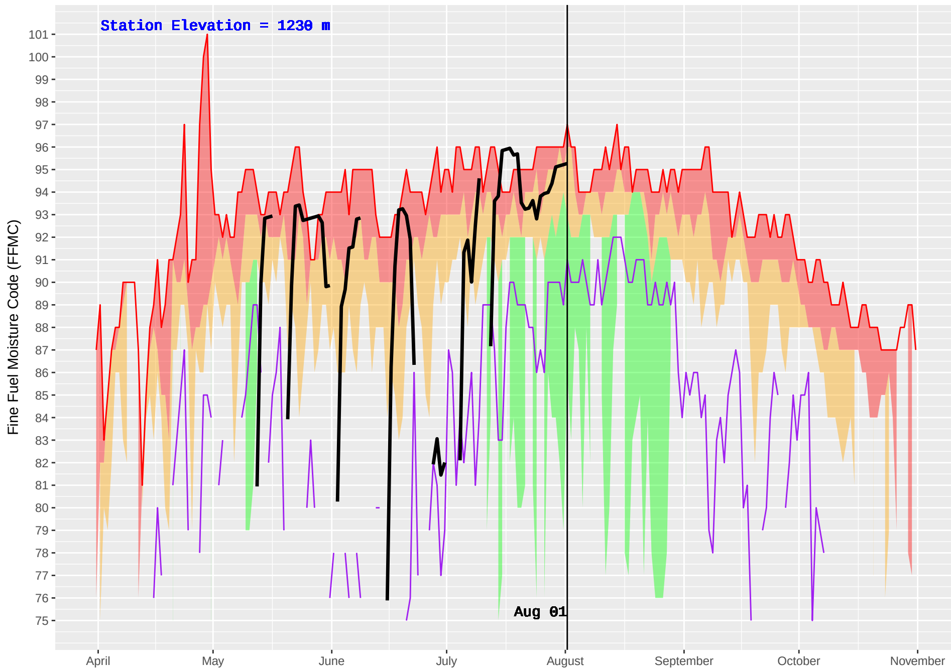
SLOCAN (406) : Historical (1992–2016) and Current (2018) Daily Fine Fuel Moisture Code (FFMC)
