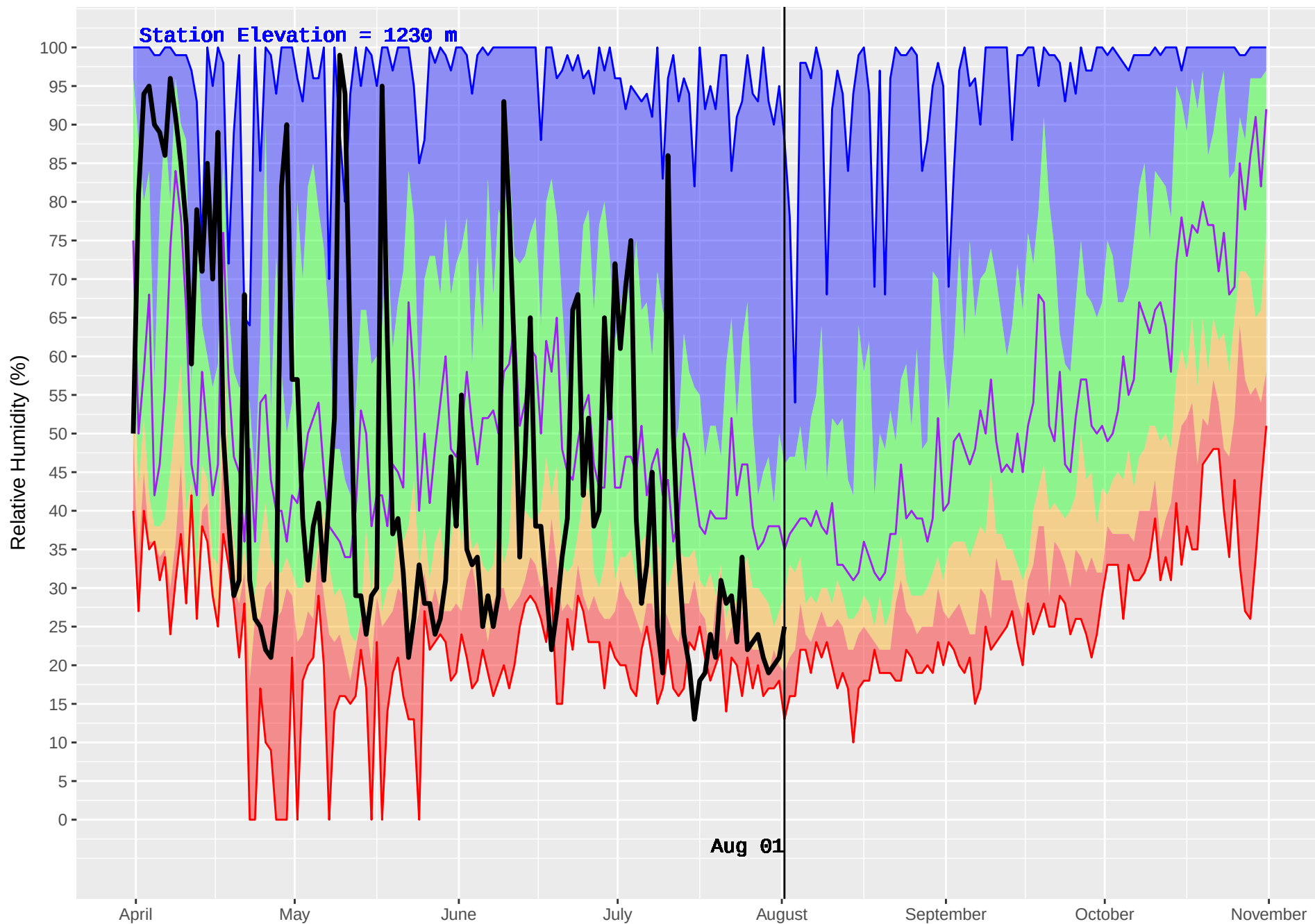
SLOCAN (406) : Historical (1992–2016) and Current (2018) Daily Relative Humidity
