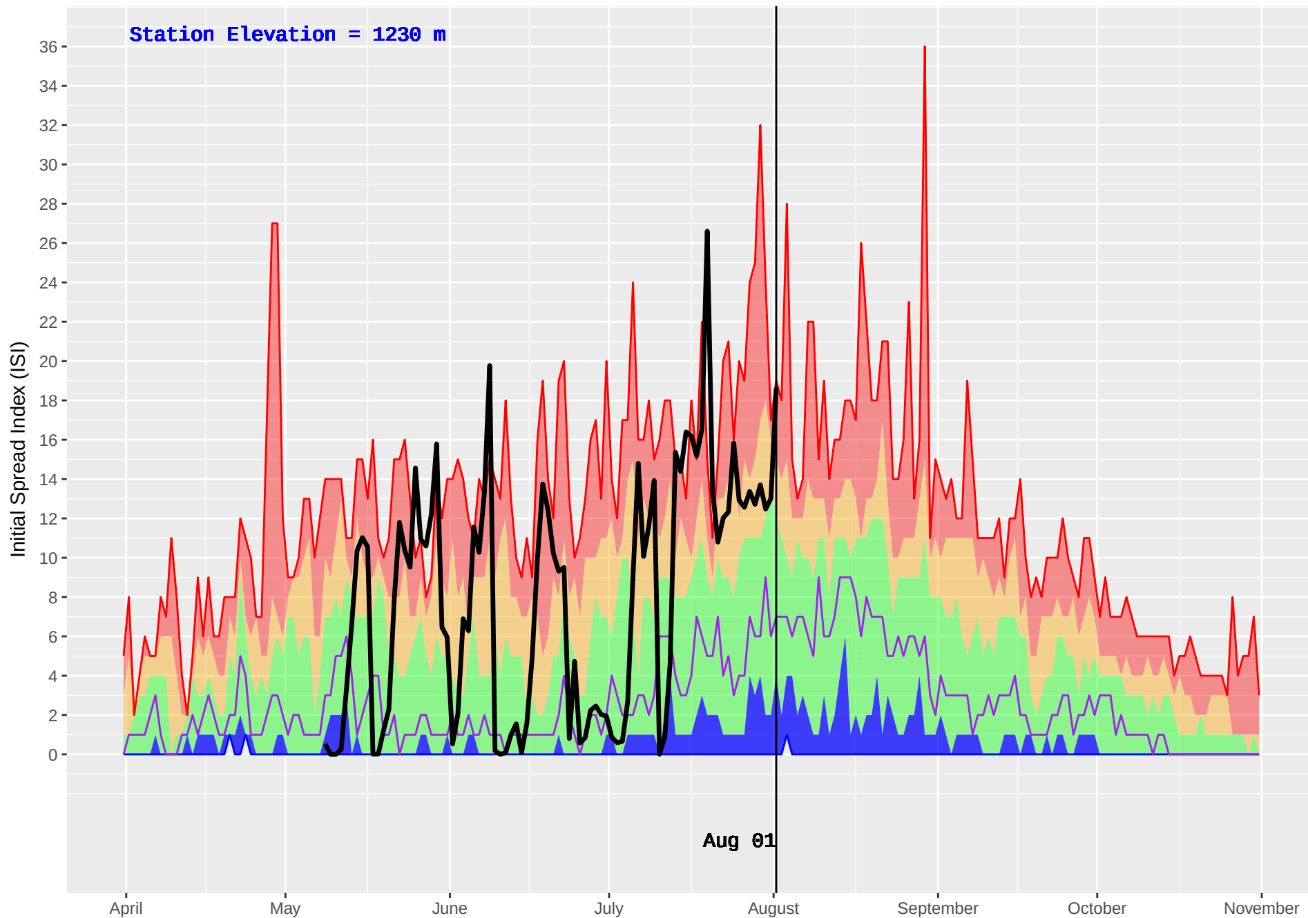
SLOCAN (406) : Historical (1992–2016) and Current (2018) Daily Initial Spread Index (ISI)
