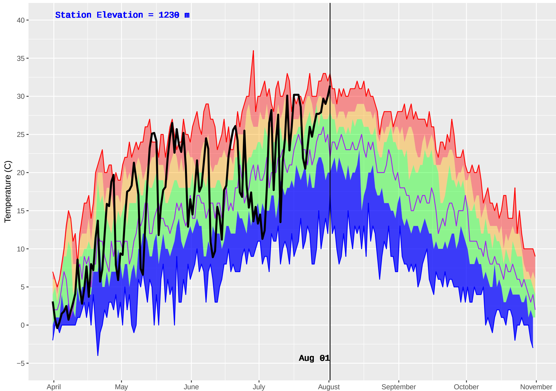
SLOCAN (406) : Historical (1992–2016) and Current (2018) Daily Temperature
